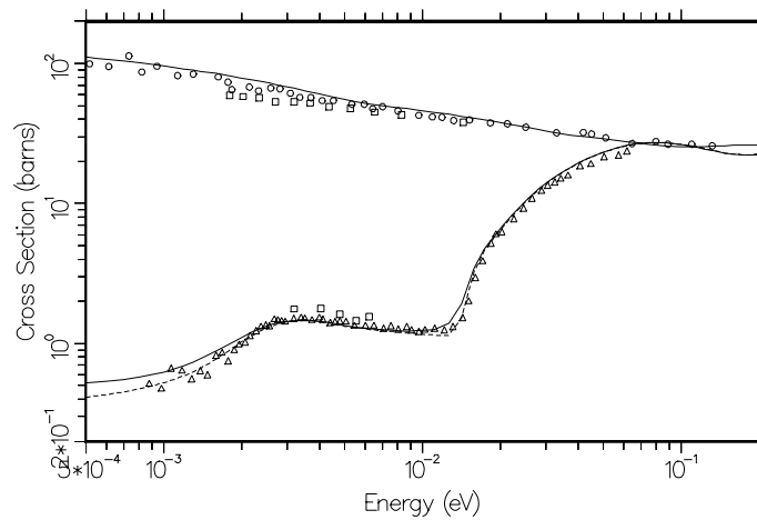
Figure 105: The cross sections for liquid ortho-hydrogen (upper curve) and liquid para-hydrogen (lower curve) at 20K are compared with experimental data[121] due to Squires (gas) at 20K (squares), Whittemore at 20K (circles), and Seiffert at 14K (triangles). The solid curves are at 20K and the dashed curve is at 14K. The sharp drop in the para cross section below 0.05 eV is due to spin coherence, and the second drop below 0.003 eV is due to intermolecular interference.
