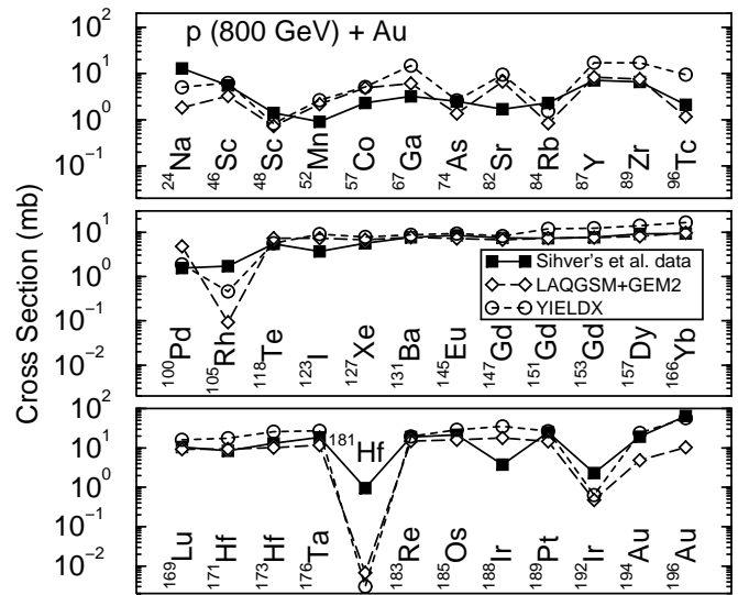
Fig. 6. Detailed comparison between experimental (Silver et al., 1992) and calculated cross sections using LAQGSM+GEM2 and YIELDX (Silberberg et al., 1998) Only every third measured product from the reaction p(800 \text{ GeV}) + \text{Au} is plotted. All cross sections shown here except for {}^{46}\text{Sc} , {}^{74}\text{As} , {}^{96}\text{Tc} , {}^{188}\text{Ir} , and {}^{192}\text{Ir} are cumulative.
