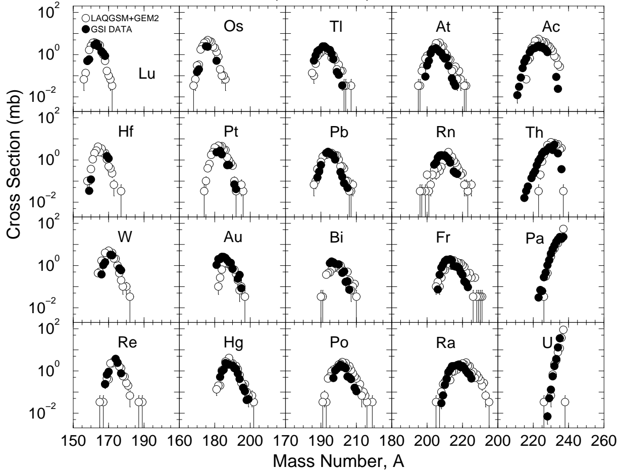
Fig. 7. Comparison of measured (Junghans, 1997; Junghans et al., 1998) cross sections of projectile fragments produced by a 950 MeV/nucleon ^{238}\text{U} beam in a copper target (black circles) with our LAQGSM+GEM2 results (open circles).
