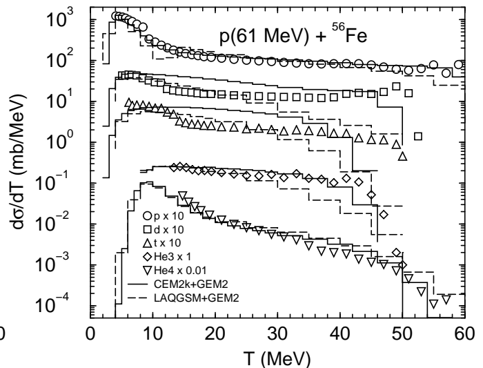
Fig. 2. Comparison of measured (Bertrand and Pelle, 1973) angle-integrated energy spectra of p, d, t, ^3\text{He} , and ^4\text{He} from 61 MeV protons on Fe with CEM2k+GEM2 and LAQGSM+GEM2 calculations.
