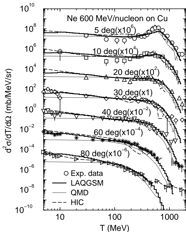
Fig. 3. Comparison of measured (Iwata et al., 2001) double differential cross sections of neutrons from 600 MeV/nucleon ^{20}\text{Ne} on Cu with our LAQGSM results and calculations by QMD and HIC (Iwata et al., 2001).
