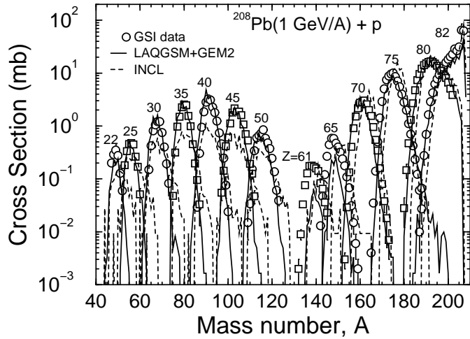
Fig. 5. Experimental (Enqvist et al., 2001) mass distributions of the cross sections of thirteen isotopes with the charge Z from 22 to 82 produced in the reaction p(1 \text{ GeV}) + {}^{208}\text{Pb} compared with our LAQGSM+GEM2 calculation and the INCL code (see the text for a description).
