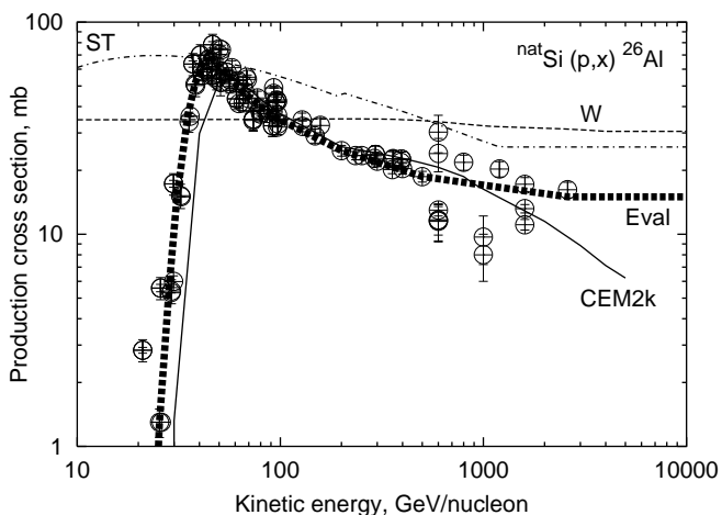
Fig. 8. Evaluated excitation function for the reaction {}^{\text{nat}}\text{Si}(p,x){}^{26}\text{Al} (thick dashed line) compared with experimental data from LANL T-16 compilation (Mashnik et al., 1999) and results by CEM2k (thin solid line) and phenomenological approximations by Webber et al. (1990) (dashed line) and by Silberberg et al. (1998) (dot-dashed line).
