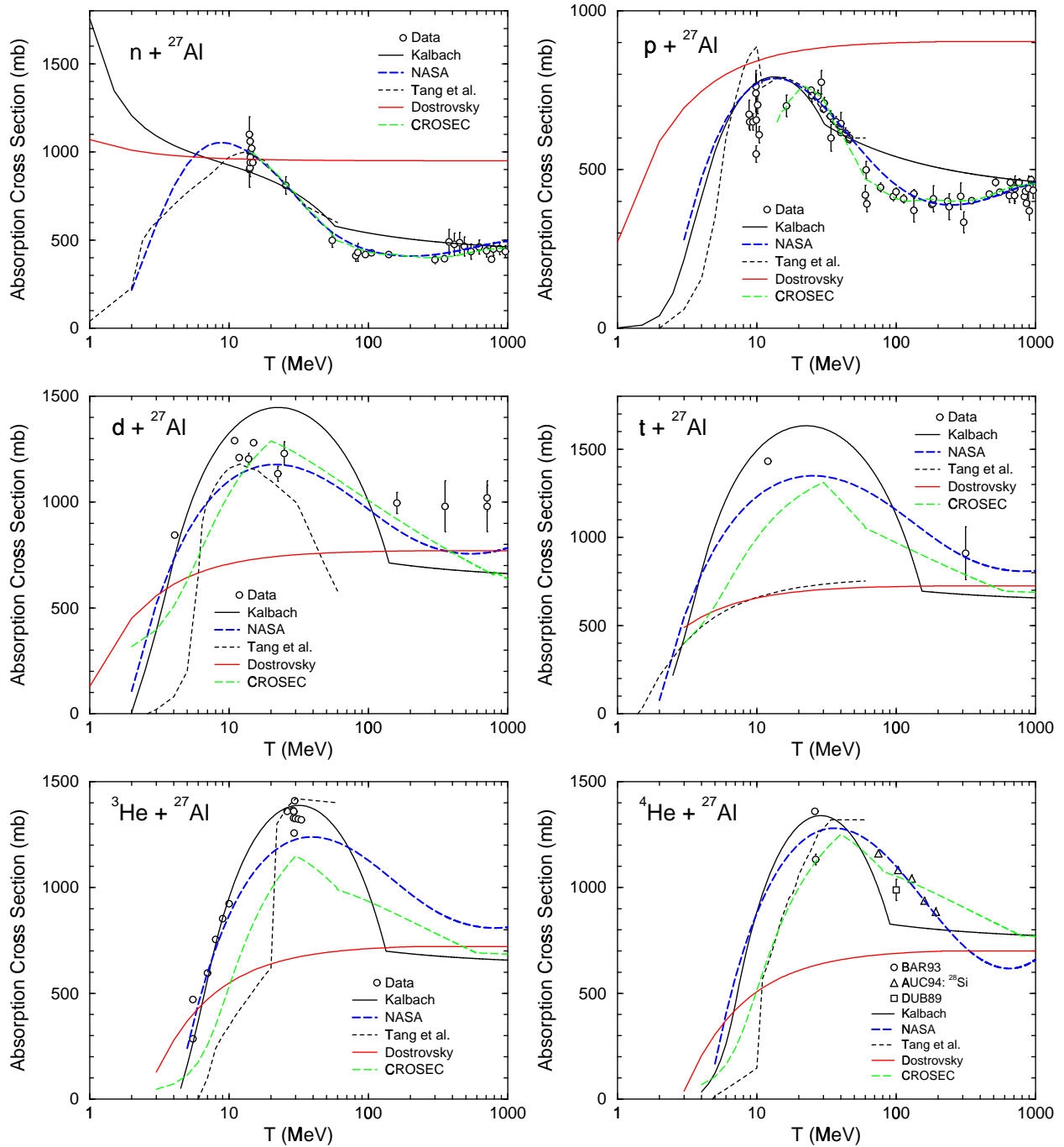
Figure 17. Comparison of experimental data on absorption cross sections for n, p, d, t, ^3\text{He} , and ^4\text{He} on ^{27}\text{Al} with the Dostrovsky et. al. 39 approximation, the NASA systematics by Tripathi, Cucinota, and Wilson 33 , a parameterization by Kalbach 34 , an approximation by Tang, Srinivasan, and Azziz 69 , and results calculated with the phenomenological code CROSEC by Barashenkov and Polanski 70 . Most of the data points (circles, either without a special label or labeled as “BAR93”) shown here are from the compilation by Barashenkov 35 ; several data points are by Auce et al. 71 (triangles labeled as “AUC94”), and a data point for ^4\text{He} is measured by Dubar et al. 72 (the square labeled as “DUB89”).
