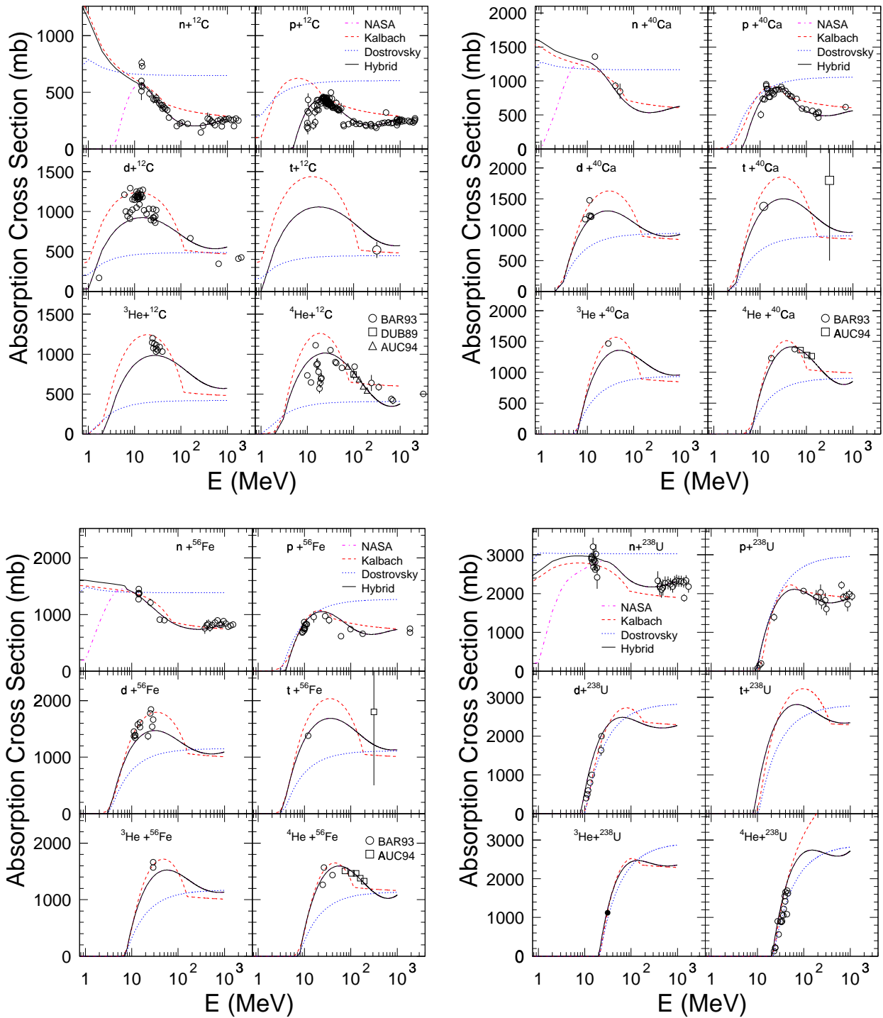
Figure 18. Inverse cross sections for n, p, d, t, ^3\text{He} , and ^4\text{He} on ^{12}\text{C} , ^{40}\text{Ca} , ^{56}\text{Fe} , and ^{238}\text{U} calculated with our routine HYBRID (black solid lines) compared with available experimental data (symbols) from the compilation by Barashenkov 35 (circles, either without a special label or labeled as “BAR93”), by Auce et al. 71 (labeled as “AUC94”), and by Dubar et al. 72 (labeled as “DUB89”). For comparison, calculations using the NASA systematics by Tripathi, Cucinota, and Wilson 33 are shown by magenta dot-dashed lines, results from the Kalbach parameterization 34 are shown with red dashed lines, and predictions by the Dostrovsky et al. 39 approximation are shown by blue dotted lines.
