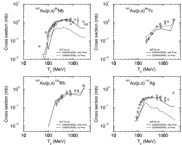
Figure 11. The same as in Fig. 8 but for the production of ^{95}\text{Nb} , ^{96}\text{Tc} , ^{102}\text{Rh} , and ^{110}\text{Ag} .
