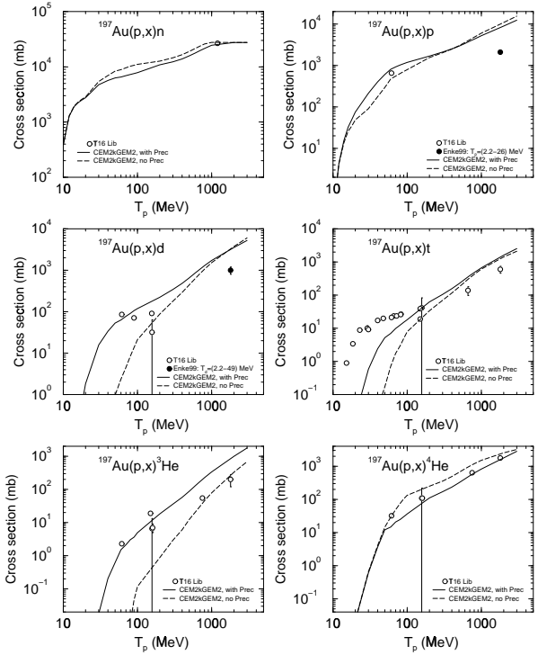
Figure 13. The same as Fig. 8 but for the production of n , p , d , t , {}^3\text{He} , and {}^4\text{He} . The complex particles are produced in CEM2k+GEM2 via evaporation and preequilibrium emission; n and p are also produced during the cascade stage.
