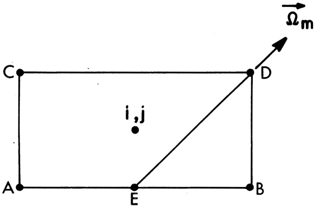
Fig. 12. (x,y) cell used to describe short characteristic method.
